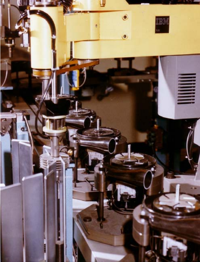
Flexible Assembly System for Motor Fan End
