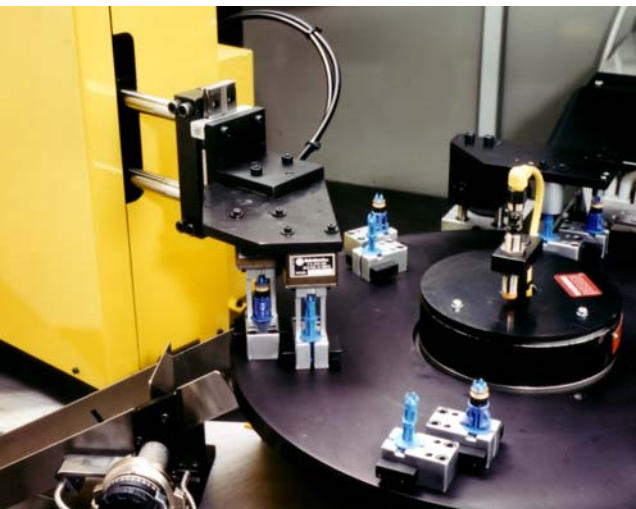
Dial Assembly System
